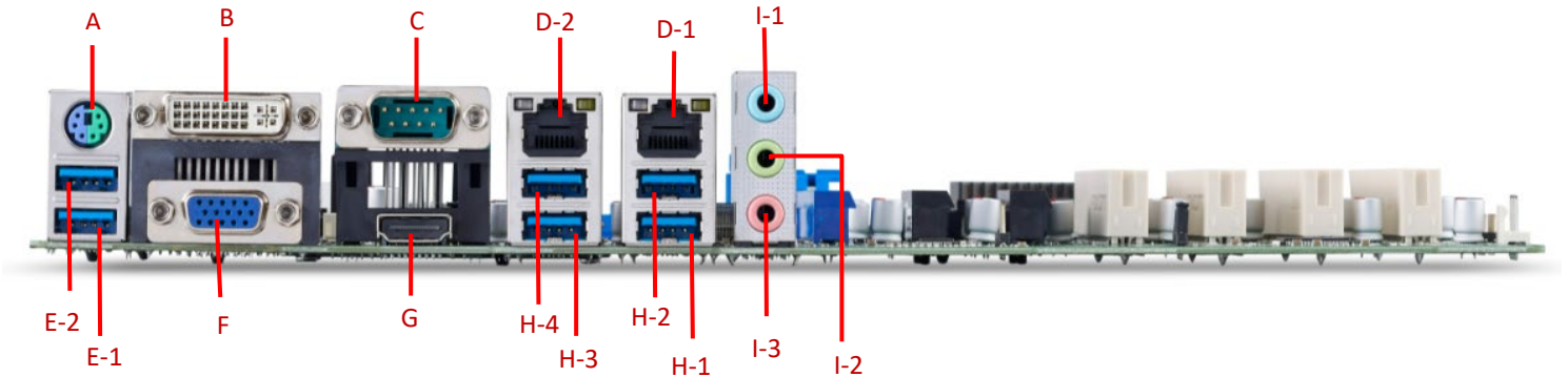
Figure 2: IO Panel Connector Locations
