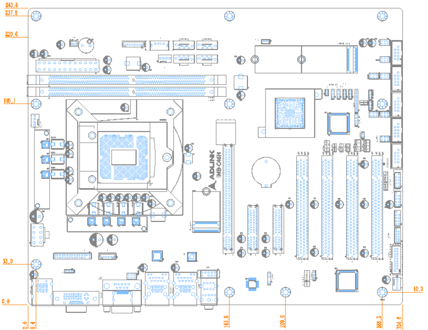
Figure 4: Mechanical Dimensions
