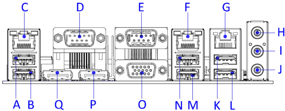
Figure 2: IO Panel Connector Locations
