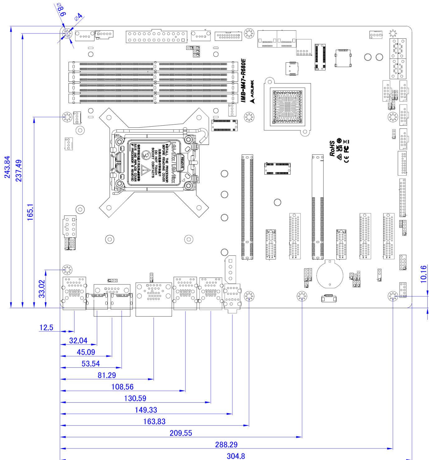
Figure 4: Mechanical Dimensions
