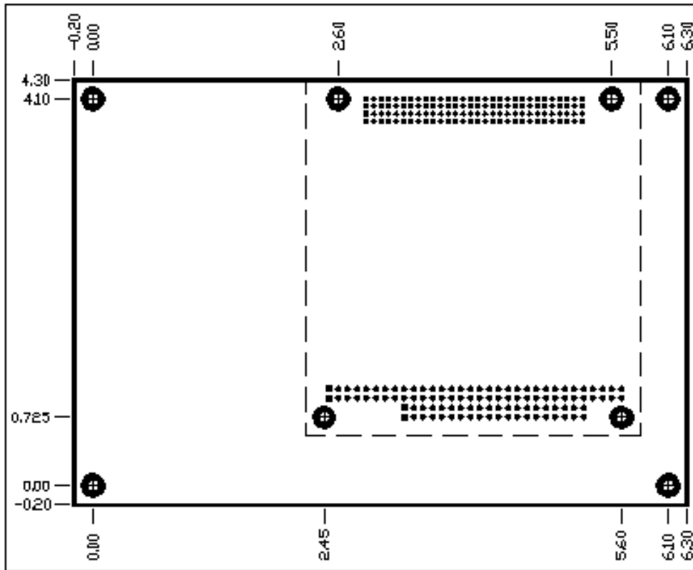
Figure 1: Board Dimensions are 4.5 x 6.5-in. (115mm x 165mm)
