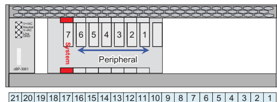
cPCIS-2651R Inside Rear View
