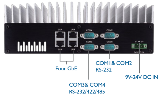
MXE-5104M Back Panel
